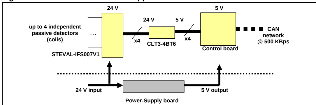
Figure 5. The boards used in the application
